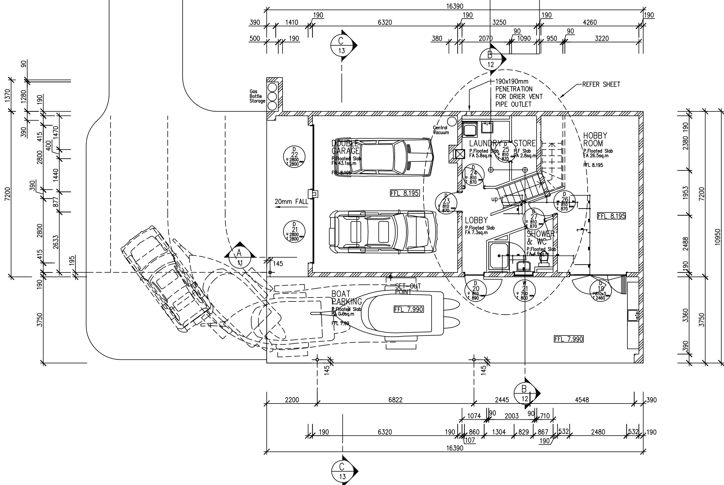
BASEMENT FLOOR LAYOUT SCALE @ A3: 1:100
