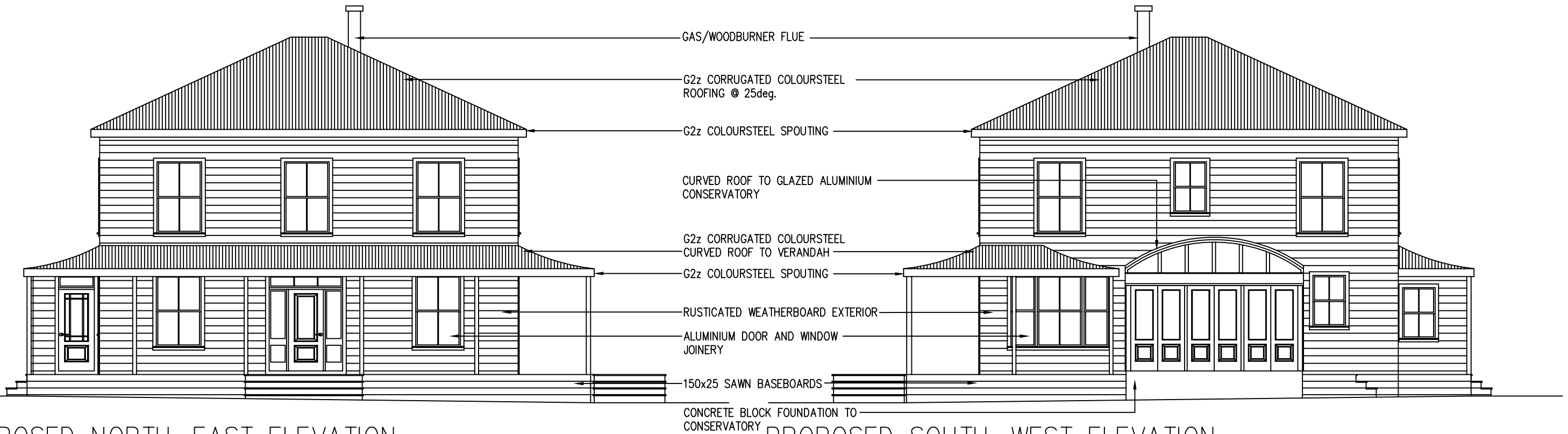
PROPOSED NORTH-EAST ELEVATION SCALE @ A3: 1:100
